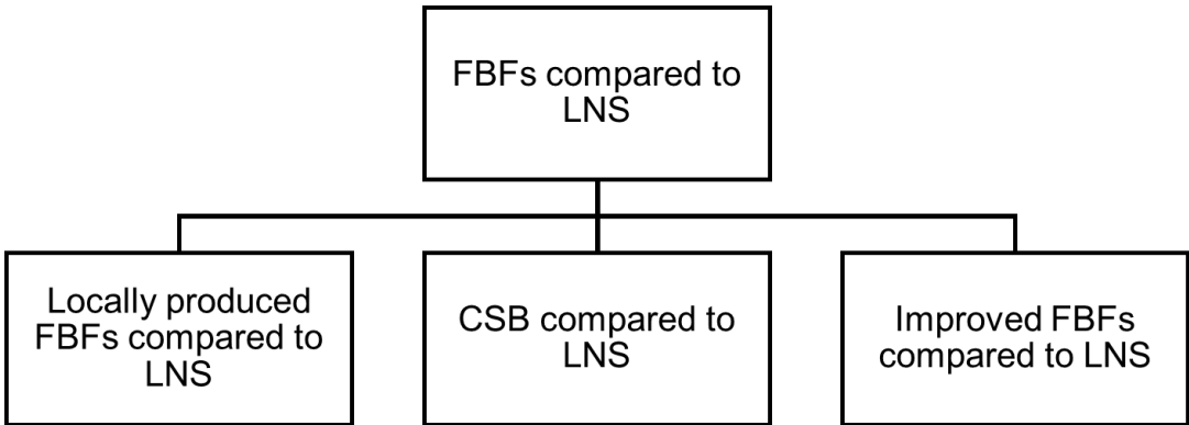
Fig. 4. Comparisons of fortified blended foods to lipid-based nutrient supplements
